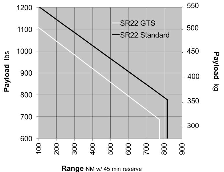
SR22 High Speed Cruise @ 8,000 Ft (180 KTAS)
