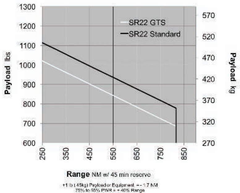
SR22 High Speed Cruise @ 8,000 Ft (180 KTAS)
