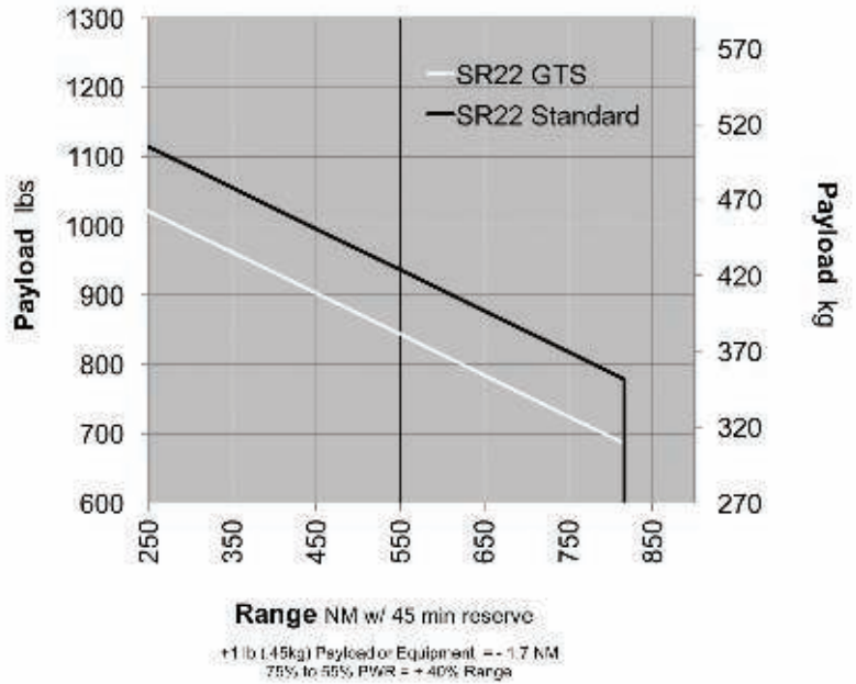
SR22 High Speed Cruise @ 8,000 Ft (180 KTAS)
