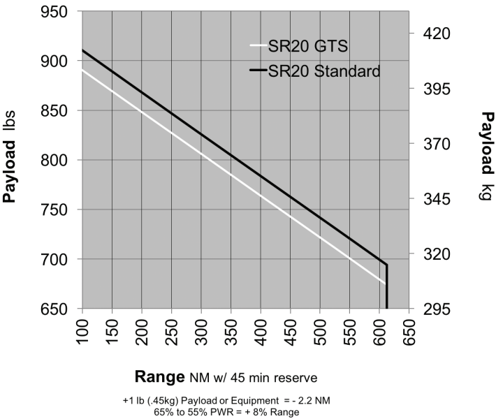
SR20 High Speed Cruise @ 8,000 Ft (145 KTAS)
