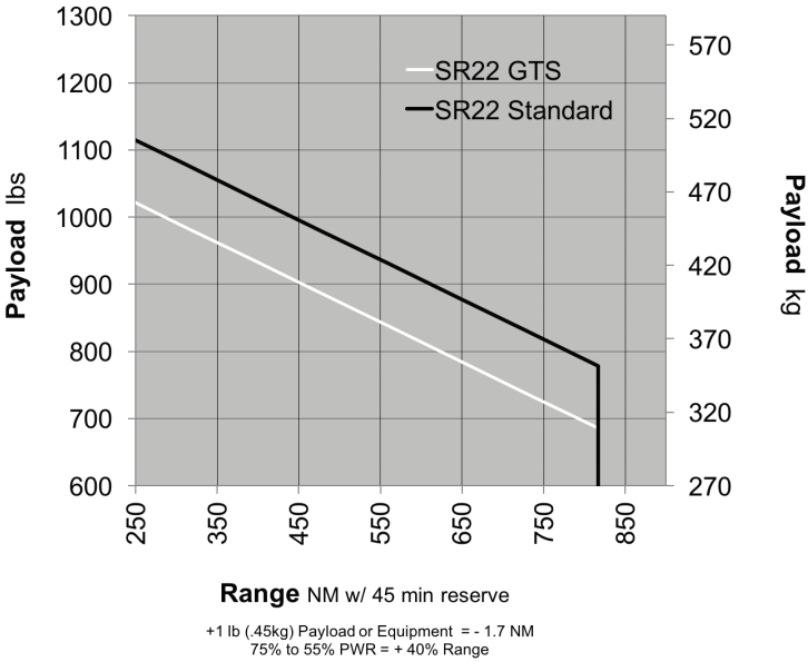
SR22 High Speed Cruise @ 8,000 Ft (180 KTAS)
